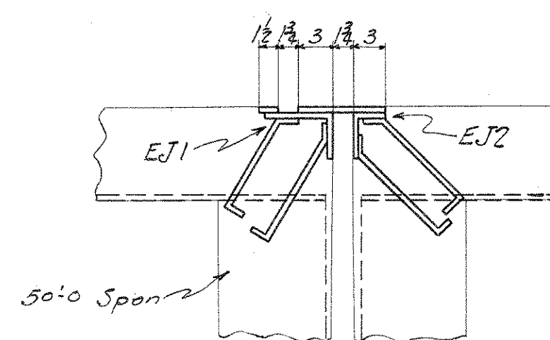
Section Thru Roadway Expansion Joints at Piers #A &amp; #G
