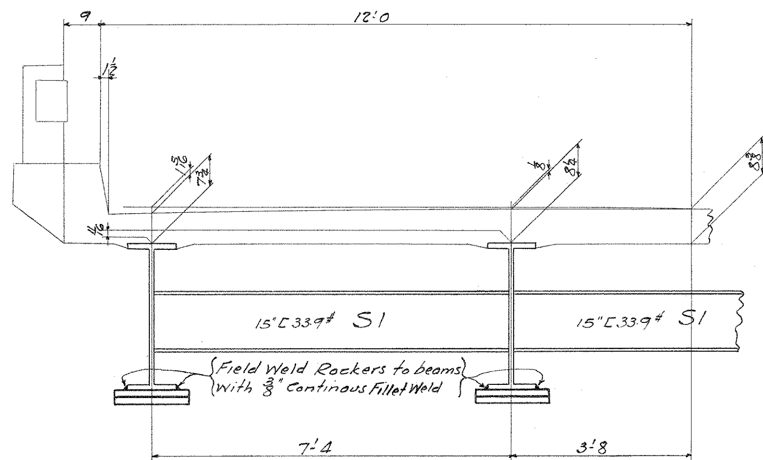
TYPICAL HALF SECTION THRU ROADWAY
