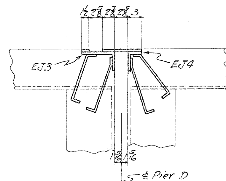
Section Thru Roadway Expansion Joint at Pier #D
