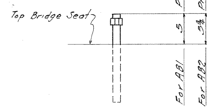
Sketch Showing Anchor Bolt Projections.
