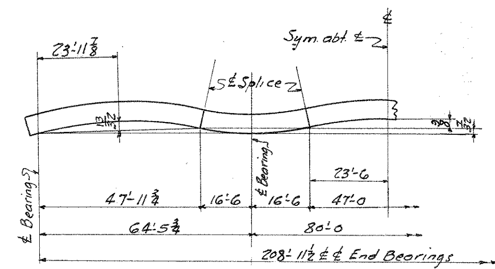
Camber Diag. for 210'-0" Continuous Stringers
