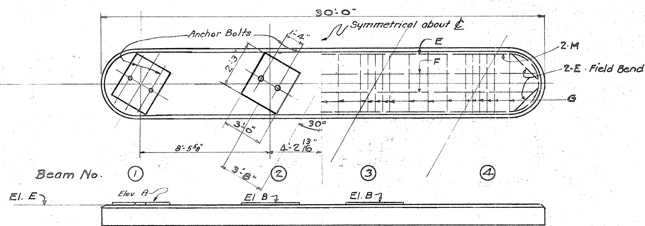
PIER B, C, E, or F Portion of pier not shown similar to Pier D
